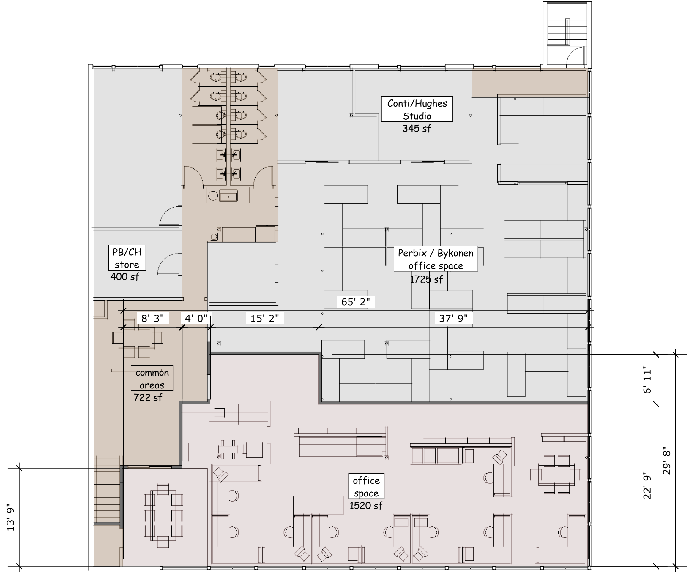
1 Office Floor Plan 1/8" = 1'-0"
